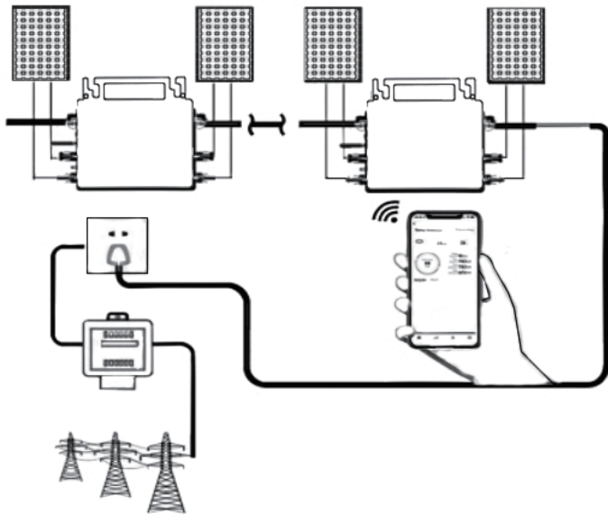
Connection diagram
